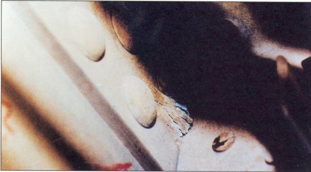
FIGURE 5-9. SPAR CHORD CORROSION
