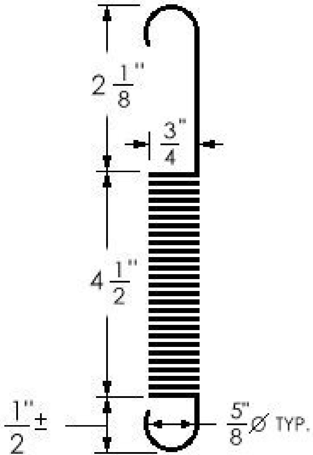
Tailwheel Over Center Locking Spring (.085" steel)
