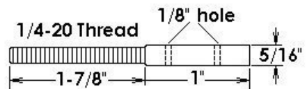
Threaded Fitting Detail
